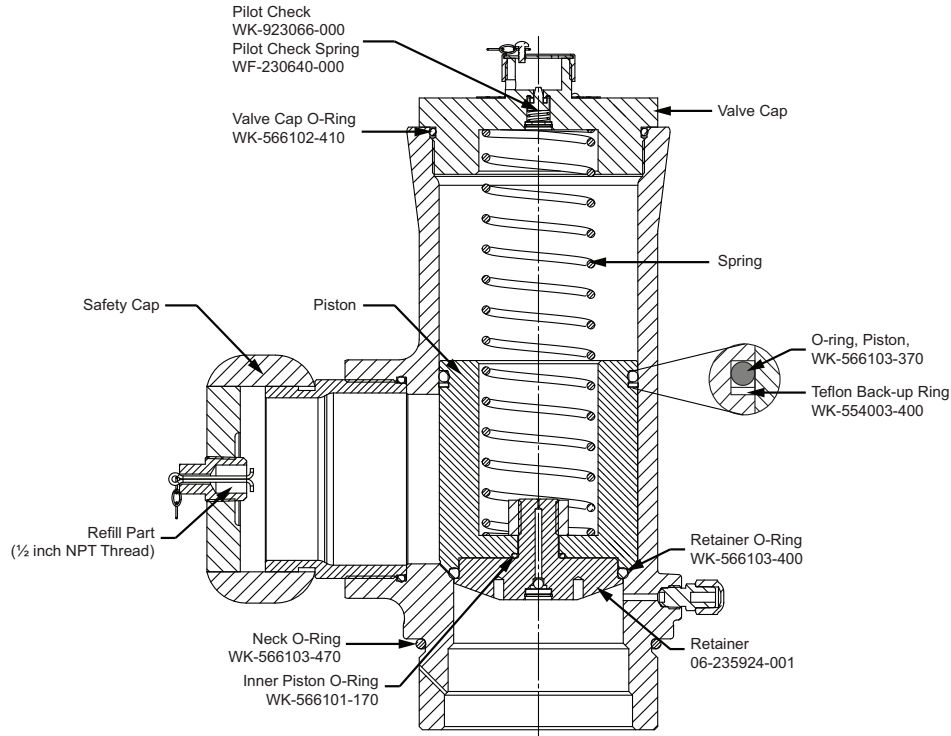
Figure 1. 3-inch Valve Assembly
